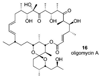
Figure 5. Structure of oligomycin A.
