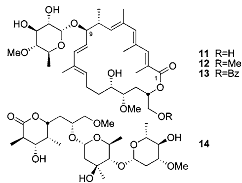
Figure 3. Structures of apoptolidin fragmentation products.
